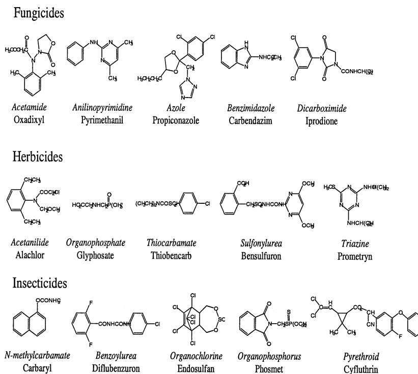
FIG. 1. Chemical structures of representative compounds of pesticides used in agriculture.
