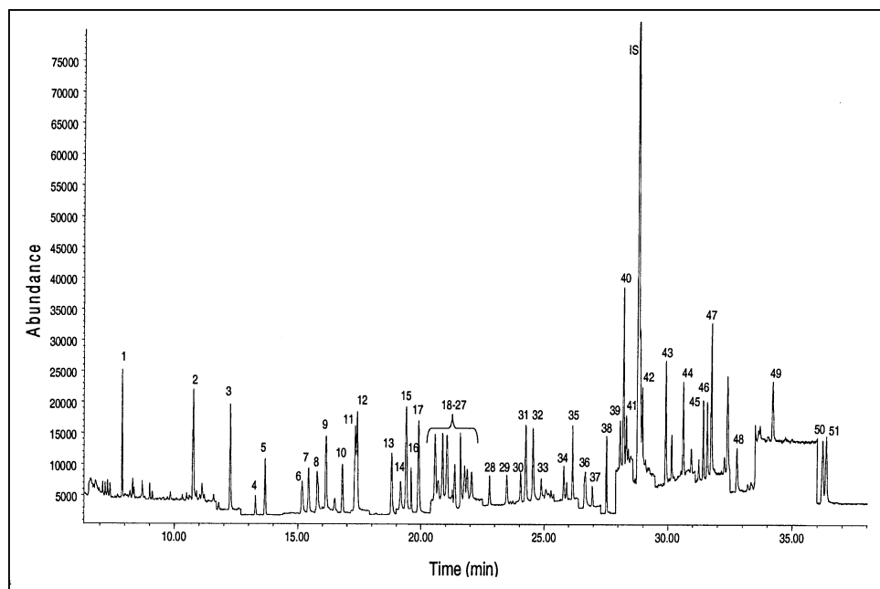
FIG. 2. GC-MS-SIM chromatogram of a grape juice sample fortified with pesticides at 0.02 \mu\text{g/mL} . Peak identification: 1: EPTC; 2: molinate; 3: propachlor; 4: ethalfluralin; 5: trifluralin; 6: simazine; 7: atrazine; 8: lindane; 9: terbuthylazine; 10: diazinon; 11: chlorothalonil; 12: triallate; 13: metribuzin; 14: parathion-methyl; 15: tolclofos-methyl; 16: alachlor; 17: prometryn; 18: terbutryn; 19: fenitrothion; 20: pirimiphos-methyl; 21: dichlofluanid; 22: aldrin; 23: malathion; 24: metolachlor; 25: fenthion; 26: chlorpyrifos; 27: triadimefon; 28: butralin; 29: pendimethalin; 30: phenthoate; 31: procymidone; 32: methidathion; 33: endosulfan I; 34: profenofos; 35: oxadiazon; 36: cyproconazole; 37: endosulfan II; 38: ethion; 39: ofurace; 40: benalaxyl; 41: endosulfan sulfate; 42: nuarimol; 43: bromopropylate; 44: tetradifon; 45: cyhalothrin; 46: fenarimol; 47: pyrazophos; 48: coumaphos; 49: cypermethrin; 50: fluvalinate tau-I; 51: fluvalinate tau-II. IS: internal standard (hexazinone).
